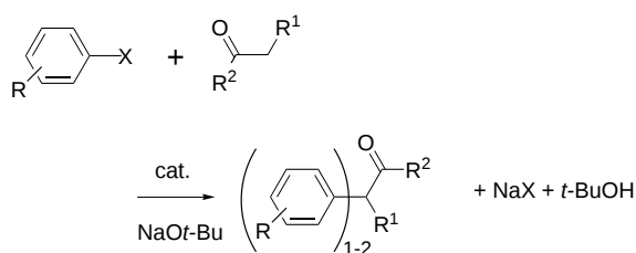
Scheme 1. \alpha -Arylation of ketones with aryl halides.
